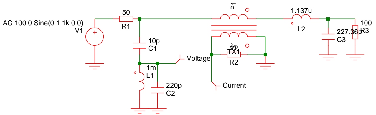
Load 100 ohm with L match
