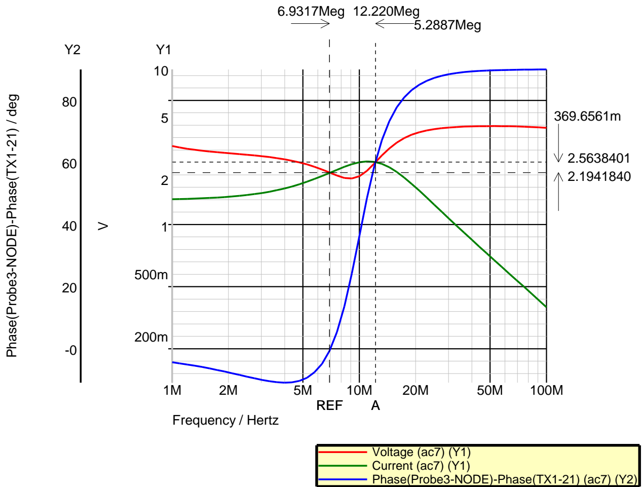
Load 100 ohm with L match
