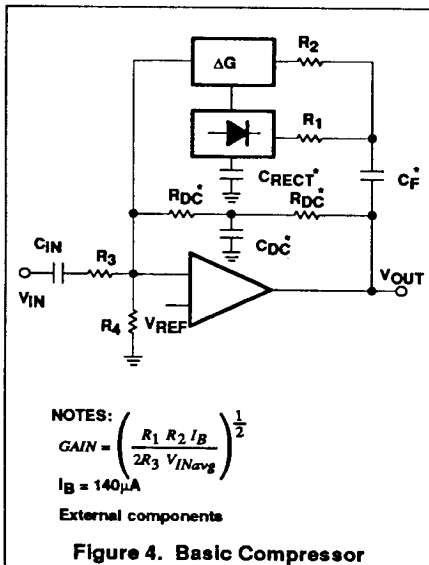
Figure 4. Basic Compressor
