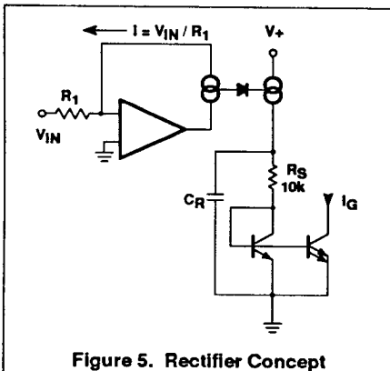
Figure 5. Rectifier Concept
