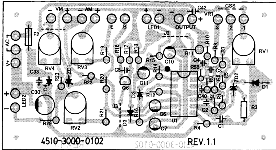
Component side
