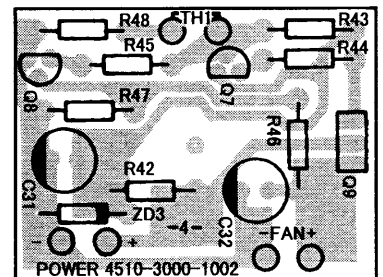
Component side
