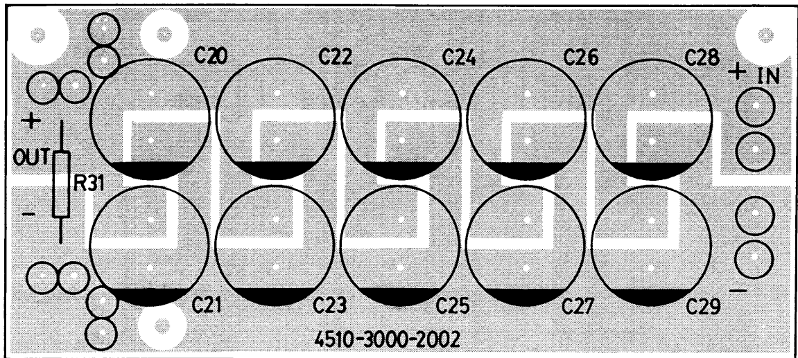
Component side
